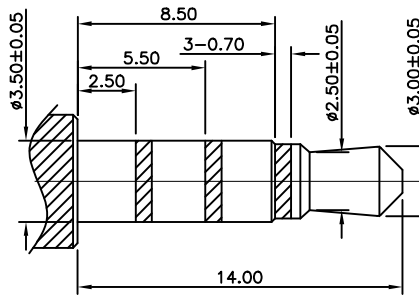
( \phi 3.50 mm 4 POLE PLUG DETAIL DRAWING)
