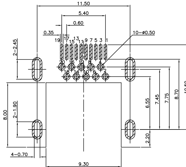
RECOMMENDED PCB LAYOUT(TOP VIEW) (THICKNESS=1.20±0.05mm) (TOLERANCE=±0.05mm)
